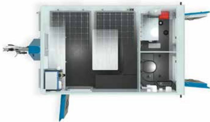
Ground lowering, anti-vandal, mobile, site accommodation unit
